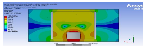
Figure 9. Sound pressure level at the enclosure for 1200 Hz
